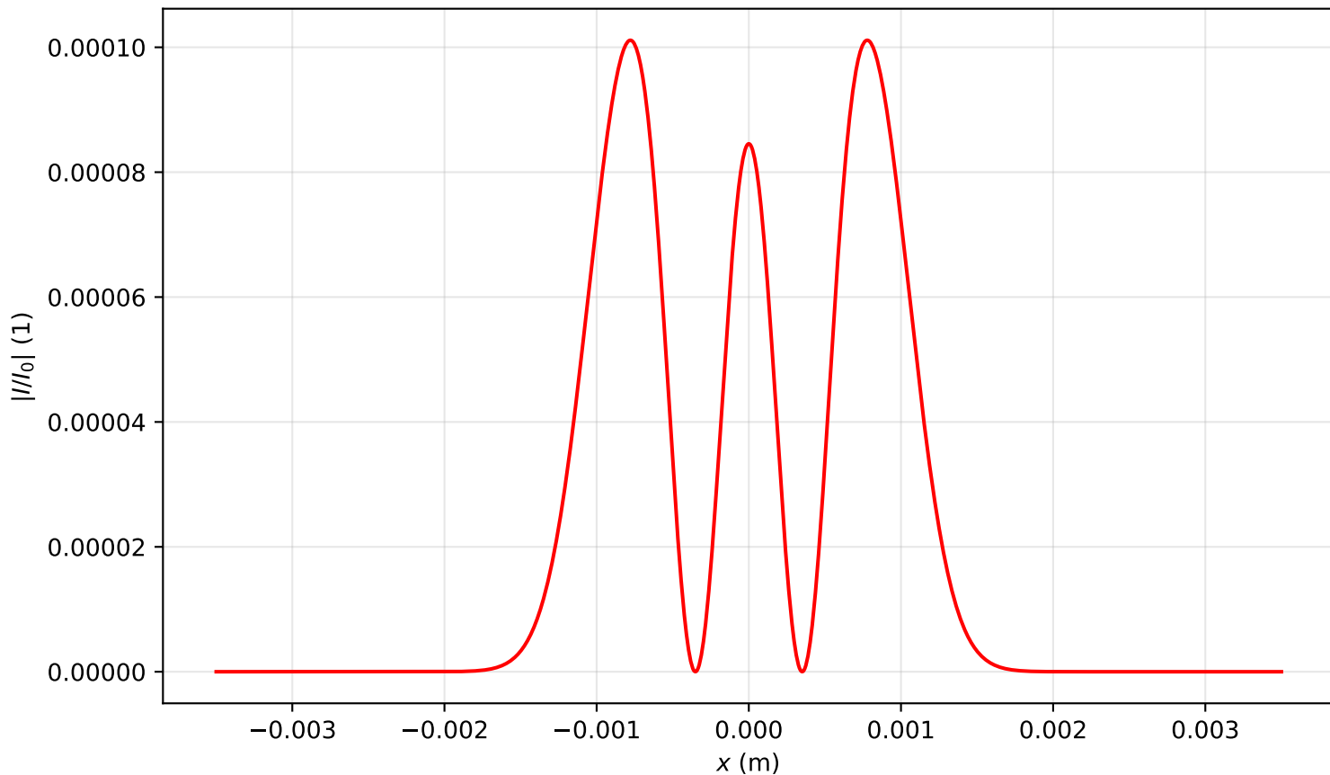
Intensity profile I(x, y = 0, z = 0.159)/I_0 , P_{in}=7.0P_{cr} , artificial time
